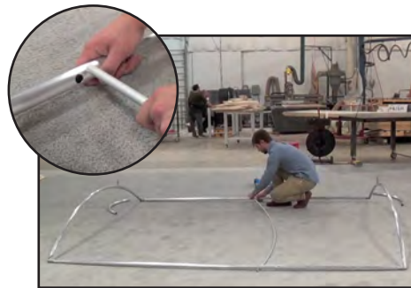
Insert support pole into hole at the BOTTOM of the frame.
