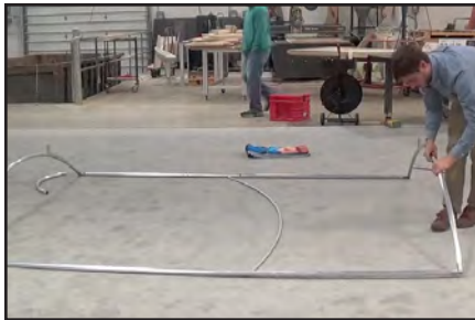
Continue connecting tubes engaging all button locks. Frame will curve on each side.
