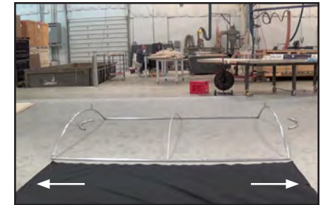
Graphic goes on face-down, holes for foot tube connection will be face-up. Begin at the TOP of the frame.
